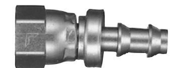
Universal Female Swivel 1/4 Hose I.D., 7/16-20 Thread Size
