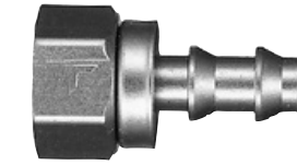
SAE Inverted Rigid Female Flare 1/4 Hose I.D., 1/2-20 Thread Size
