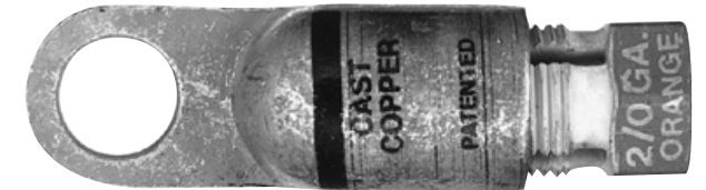
Starter/Cable Lug 2/0 Ga., 1/2 Stud Orange Color Code
