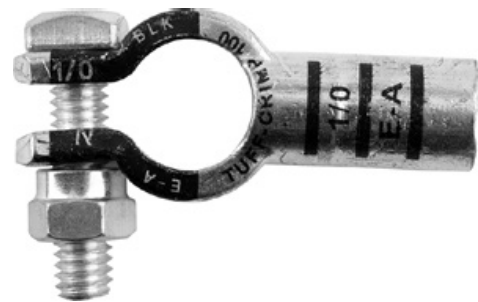
Straight Post-Top Terminal 1/0 Ga. Negative
