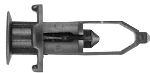
Rear Bumper Cover Retainer Toyota 18mm Head Dia., 28mm Stem Length Fits into 9mm Hole
