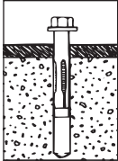
2. Insert anchor
