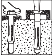
3. Tighten
